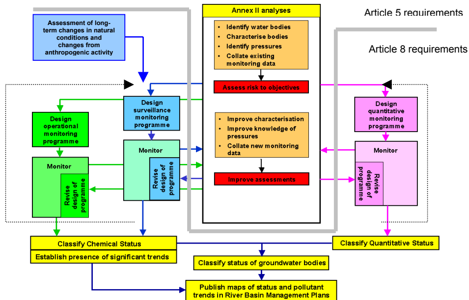
Figure 2 Schematic diagram illustrating the relationship between Article 5 and Article 8 in the design of groundwater monitoring programmes
